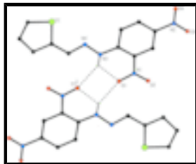
Fig. 2. View showing the N-H...O hydrogen bonds building a R_2^2(12) graph set motif. Hydrogen bonds are shown as dashed lines.
