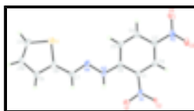
Fig. 1. Molecular view of the title compound with the atom-labeling scheme. Displacement ellipsoids are drawn at the 30% probability level. H atoms are represented as small spheres of arbitrary radii.
